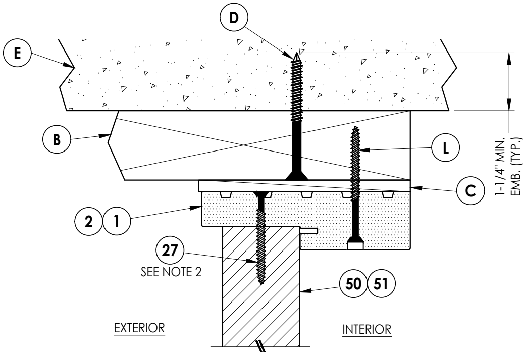
3 VERTICAL CROSS SECTION
