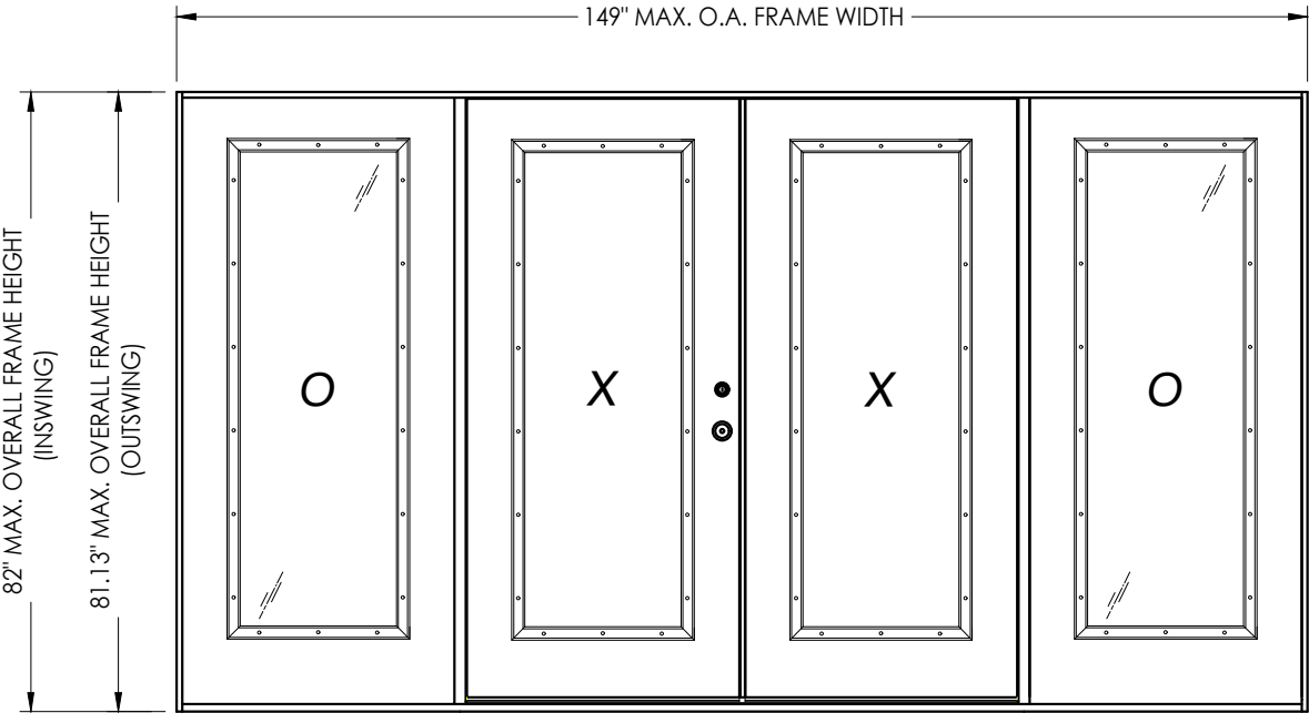
OXXO CONTINUOUS HEAD & SILL
